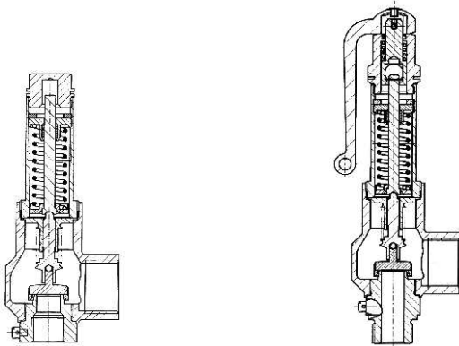
Part No. 06800 (inlet female thread) Part No. 06801 (inlet male thread)
